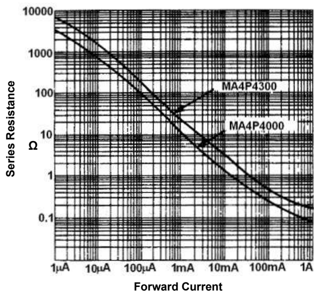
Series Resistance at 100 MHz vs. Forward Current MA4P4000, MA4P4300 Series
