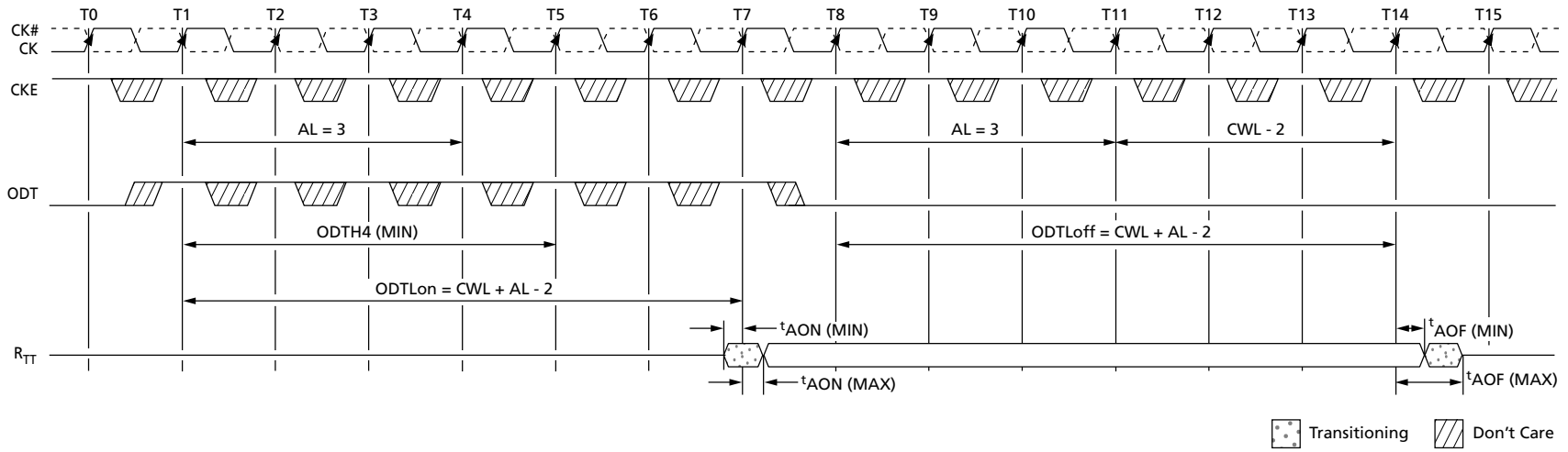
Figure 112: Synchronous ODT
