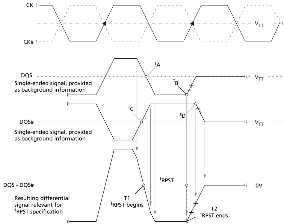
Figure 79: t_{RPST} Timing
