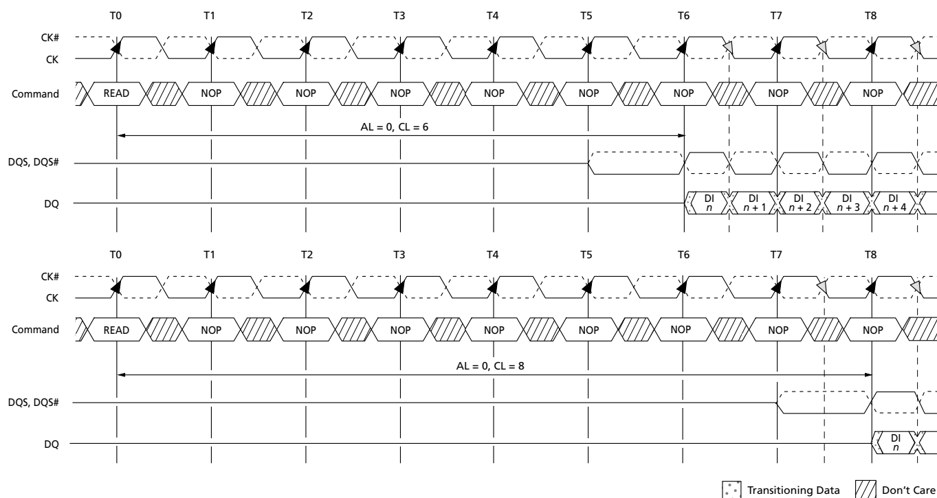
Figure 51: READ Latency
