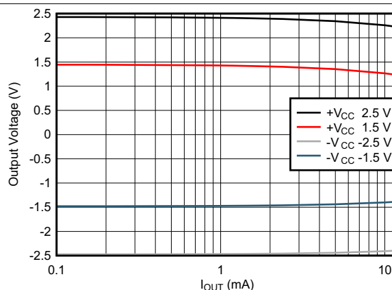
Figure 56. Output Saturation Voltage vs Load Current
