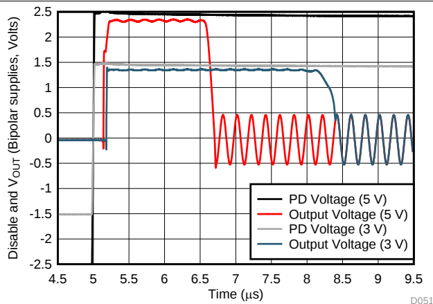
Figure 51. Turnon Time to Sinusoidal Input
