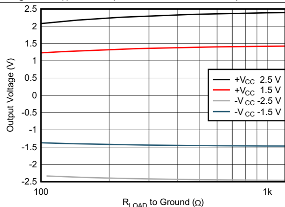
Figure 55. Output Voltage Swing vs Load Resistor
