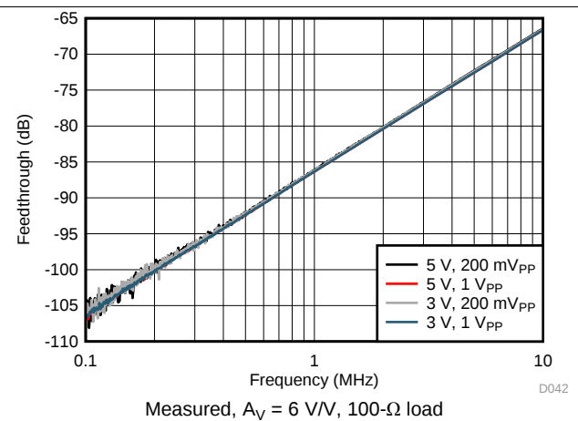
Figure 42. Disabled Isolation Noninverting Input to Output
