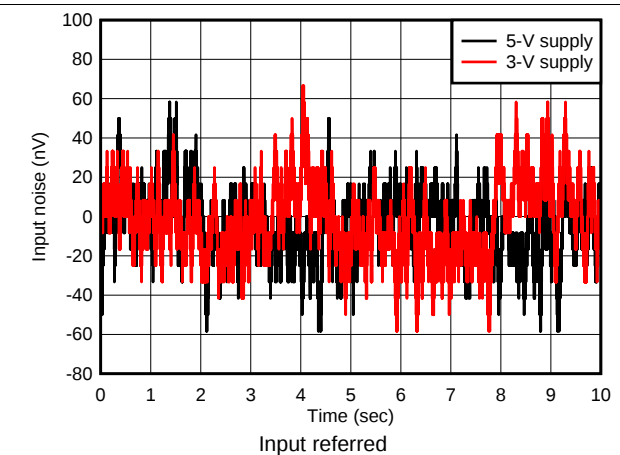
Figure 40. Low-Frequency Voltage Noise
