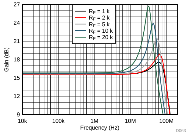
Figure 63. Frequency Response With Various Feedback Resistor Values
