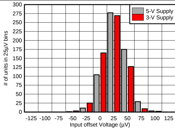
Figure 43. Input Offset Voltage Distribution
