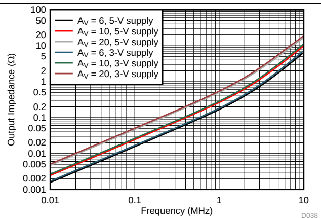
Figure 38. Closed-Loop Output Impedance
