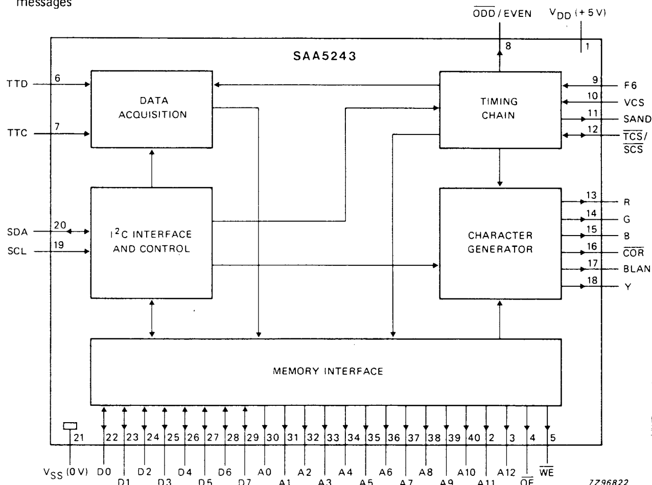
Fig.1 Block diagram.
