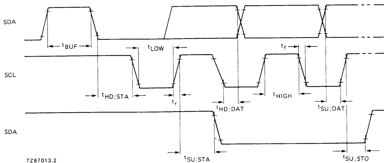
Fig.8 I 2 C-bus timing.
