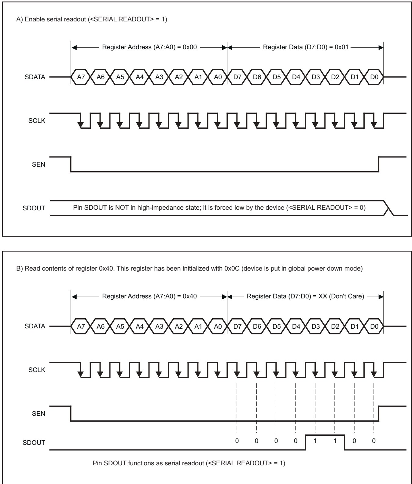
Figure 10. Serial Readout
