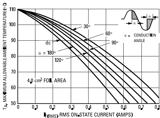
Figure 6. Current Derating, 2.0 cm Square Pad Reference: Ambient Temperature
