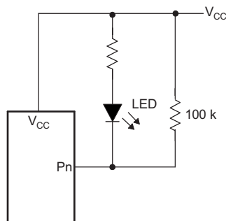
Figure 9-2. High-Value Resistor In Parallel With Led
