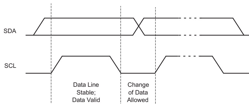
Figure 8-4. Bit Transfer
