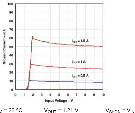
Figure 10. TL1963A Ground Current vs Input Voltage
