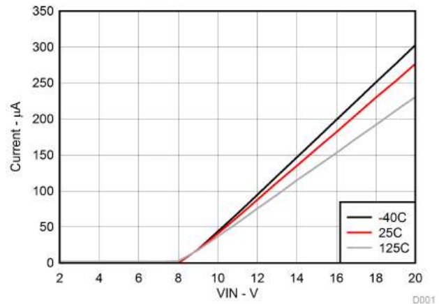
Figure 14. Quiescent Current in Shutdown vs Input Voltage
