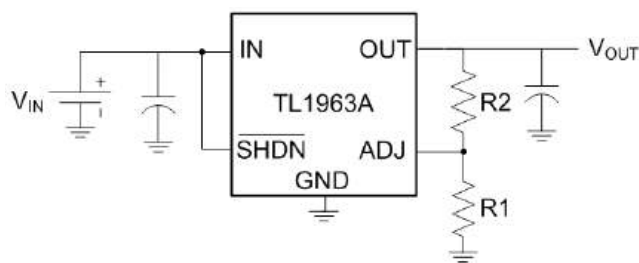
Simplified Schematic
